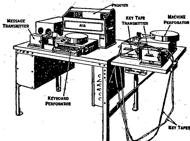
FIG. 12.—A PRINTING TELEGRAPH CIPHER MACHINE
