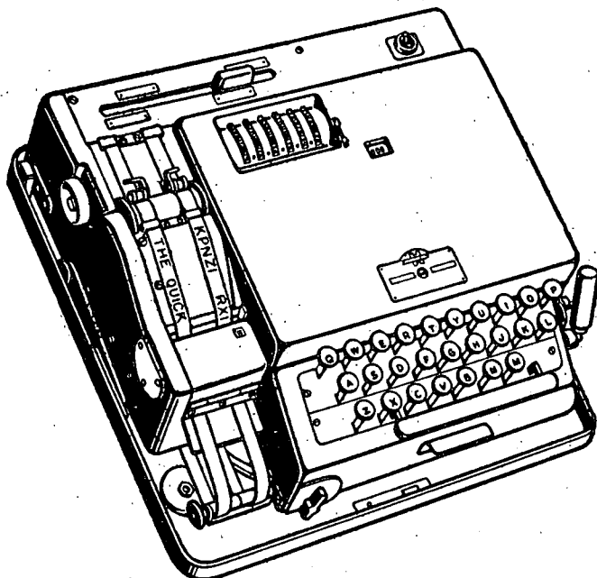
FIG. 11.—THE CRYPTODEVICE OF FIG. 9 EQUIPPED WITH A KEYBOARD AND DRIVEN BY AN ELECTRIC MOTOR. THE TWO MACHINES ARE CRYPTOGRAPHICALLY INTERCOMMUNICABLE. THE OPERATING LEVER AT RIGHT IS USED IN CASE OF POWER FAILURE
