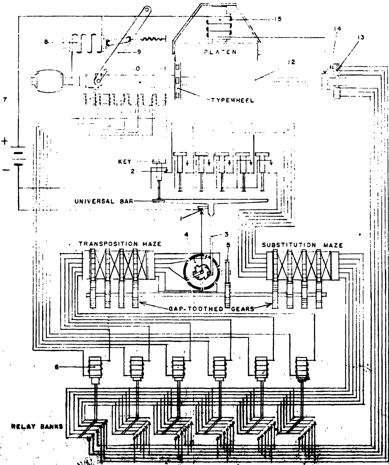
KOCH CIPHER MACHINE
